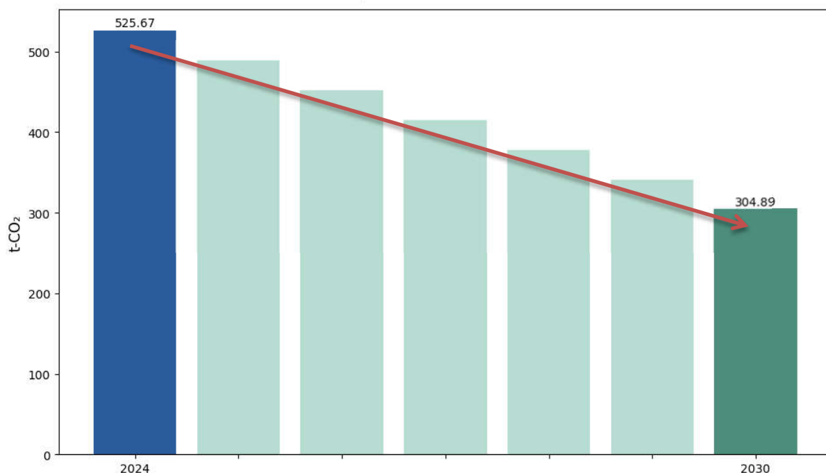
CO 2 emissions trends (2024 standard → 2030 42% reduction target)
